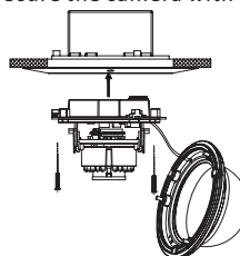
Figure 2-8 Fix the Camera to the Gang Box
